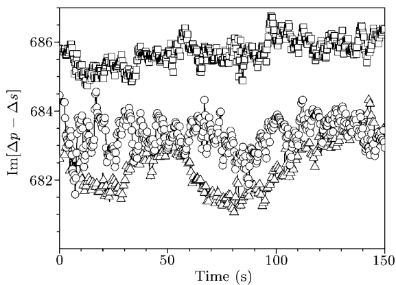
Fig. 2. \text{Im}(\Delta p - \Delta s) intensities of three spots on the bare glass. Open squares: first spot; open triangles: second spot; open circles: third spot.
